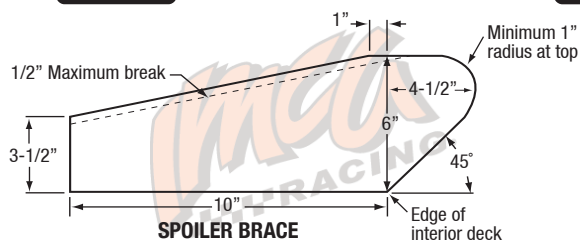
SPOILER BRACE
